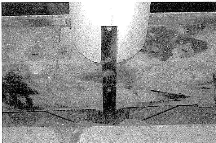
▲側柱と腰桁
